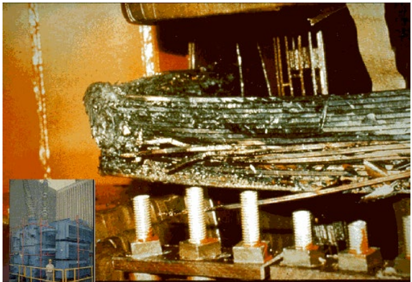
Geomagnetic Storm Induced Transformer Damage
